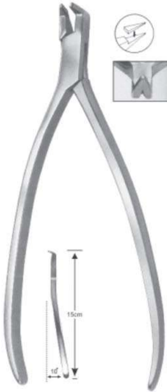
ZS-61-4020-TC Distal End Safety Cutter -Slim (Long Handle)
